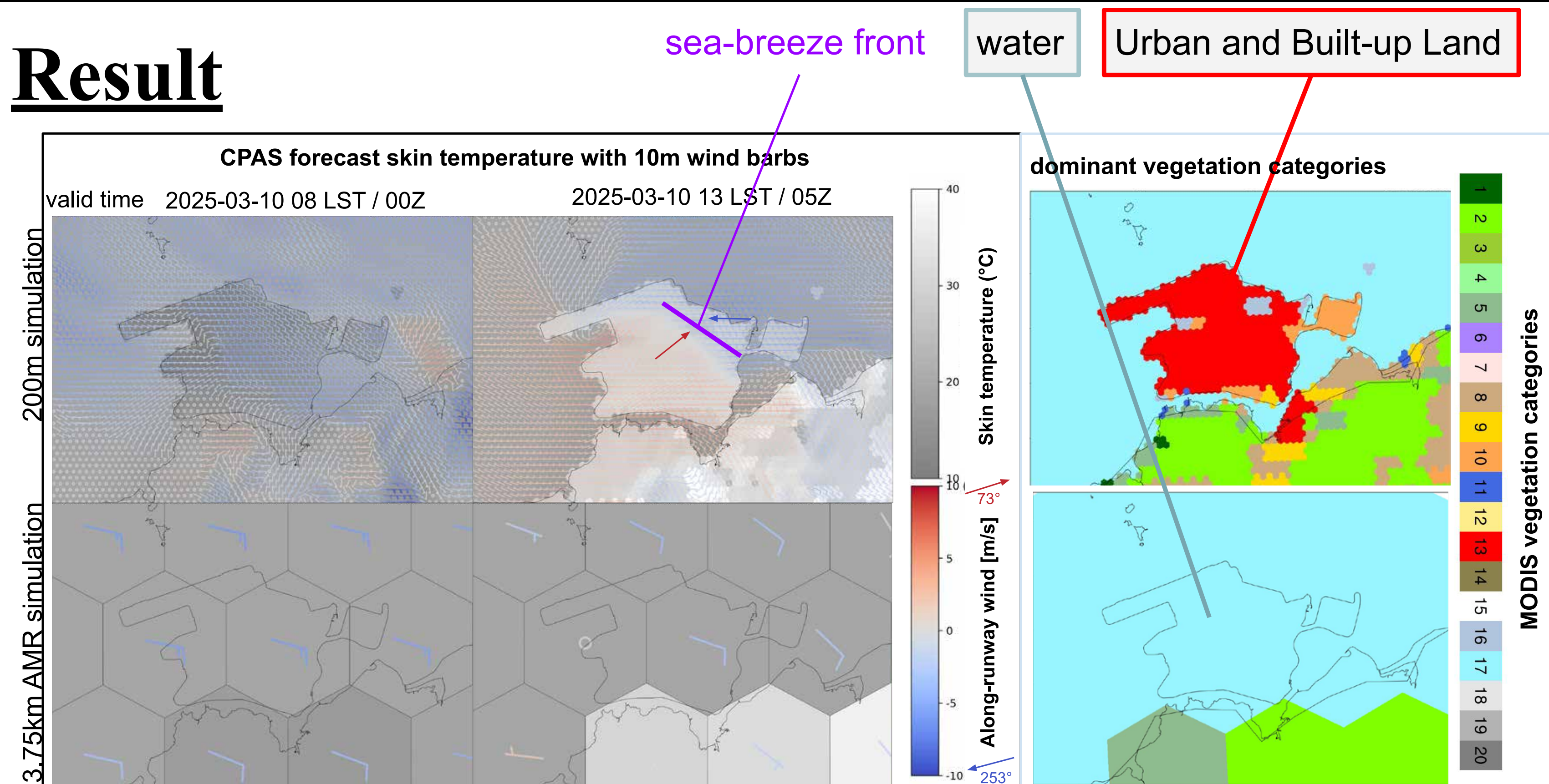
Fig. 2: Impact of grid resolution on boundary layer convergence and surface forcing.
